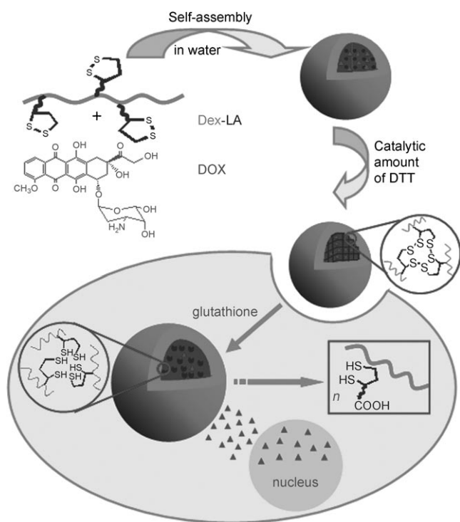
Figure 1. Schematic illustration of reversibly stabilized, multifunctional dextran nanoparticles. Dex-LA, readily obtained by coupling lipoic acid to dextran, forms nanoparticles in water. The addition of a catalytic amount of DTT yields stable nanoparticles through a cross-linking of the core. In cancer cells, fast de-cross-linking takes place as a result of a high concentration of glutathione (GSH) tripeptides, which effects rapid release of the drugs (shown as triangles) to the cell nucleus. The nanoparticles will eventually be degraded to the nontoxic products dextran and lipoic acid.
